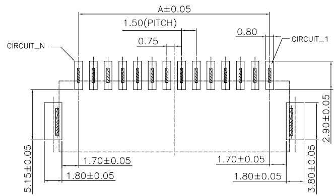
RECOMMENDED PCB LAYOUT TOLERANCE:±0.05 THICKNESS : 0.8-1.6mm
